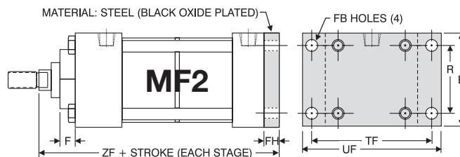
1.50" - 6.00" Bores
