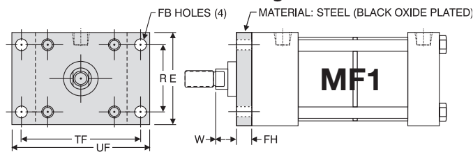
1.50" - 6.00" Bores
