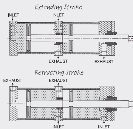
Model MSE/MSR 2 Stage Shown
